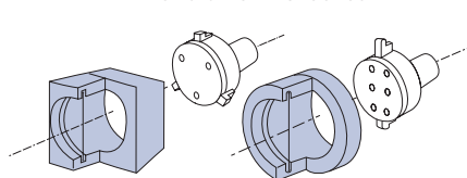
2 and 3 Point Grooves
