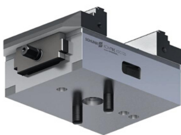
Mounting with two screws
